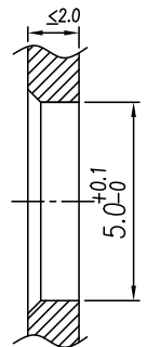
Panel cut-out
